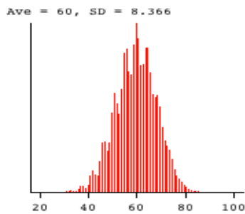
Histogram 1
