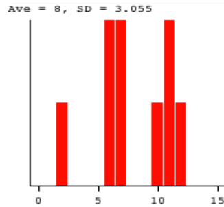
Histogram 2
